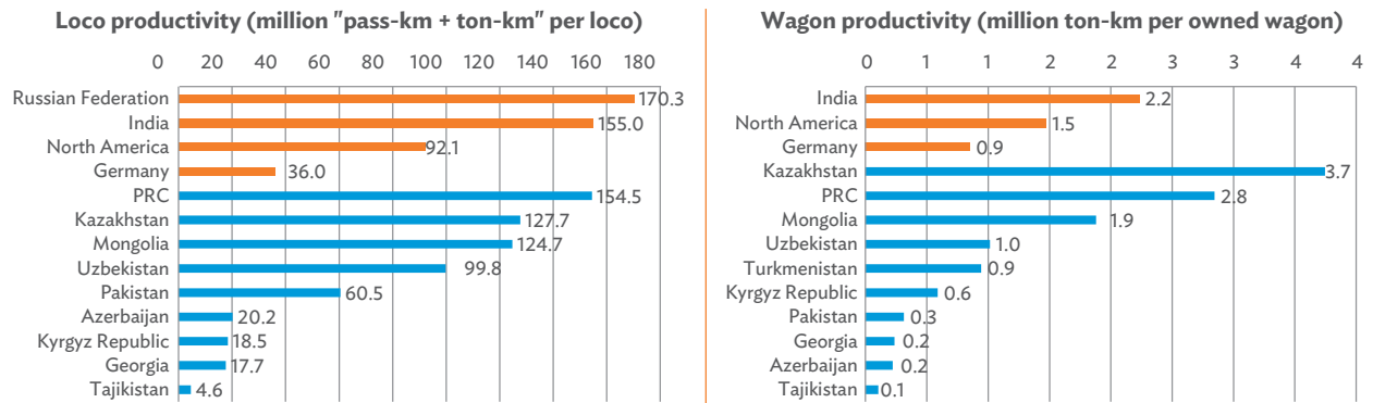
Figure 4.6: Comparison of Locomotive and Wagon Productivity in Kazakhstan, other CAREC Member Countries and other Leading Railway Countries
